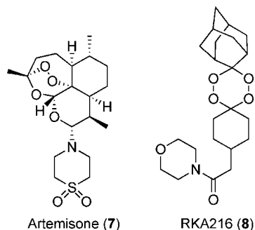
Figure 3. Structures of artemisone and 8 (RKA216).
