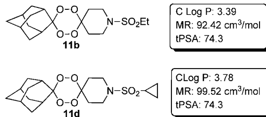
Figure 4. Calculated log P and PSA of lead compounds 11b and 11d .
