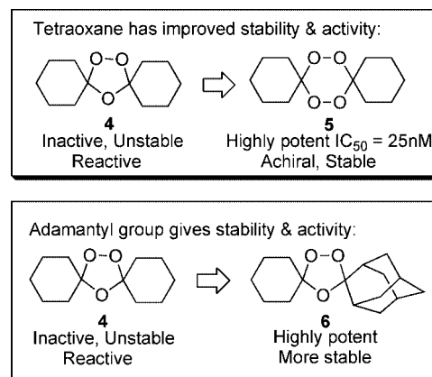
Figure 2. Stability and reactivity of endoperoxides 4–6 .
