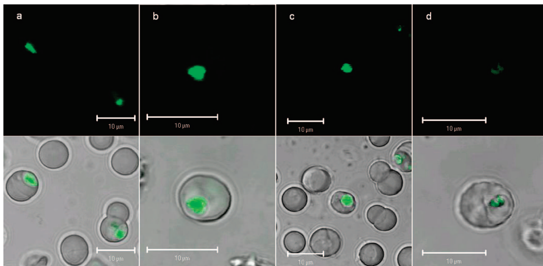
Figure 6. Confocal microscope images of infected red blood cells with NBD conjugates (1 \mu\text{M} ) in the presence or absence of DFO (100 \mu\text{M} ). The NBD-labeled compound was added 10 min before imaging. For imaging experiments using DFO, the parasite cultures were preincubated at 37 ^\circ\text{C} for 30 min with DFO prior to use. After uptake of drug, the perfusion chamber was washed with 5000 \times its volume of media to examine the retention of fluorescence: Tetraoxane–NBD adduct 33 without DFO before (a) and after wash (b) and with DFO (100 \mu\text{M} ) before (c) and after wash (d).
